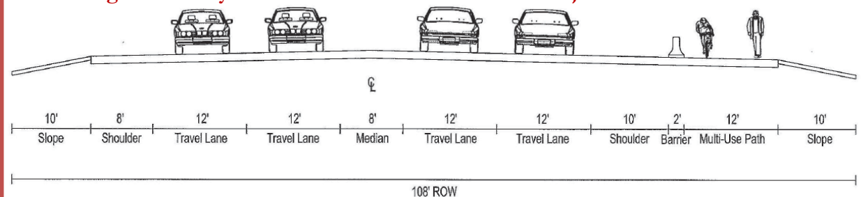
Figure 13: Very Constrained 4-Lane Section with adjacent Multi-Use Path
